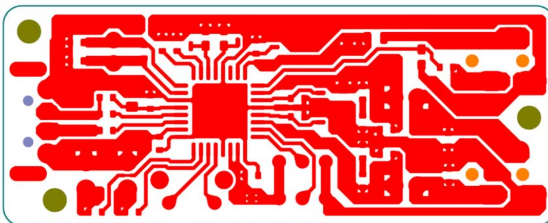
Figure 5-4. DEM-PCM2912 EVM Board Layout—Inner View
